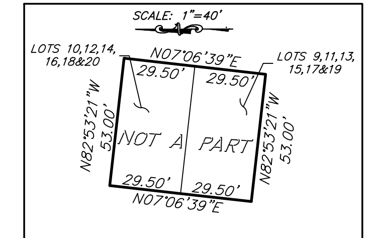
DETAIL FOR LOTS 9-20 TRACT NO. 15-002
